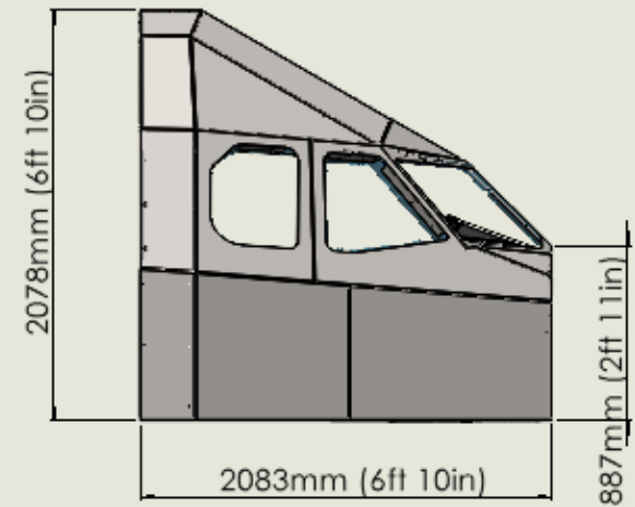
RIGHT VIEW
