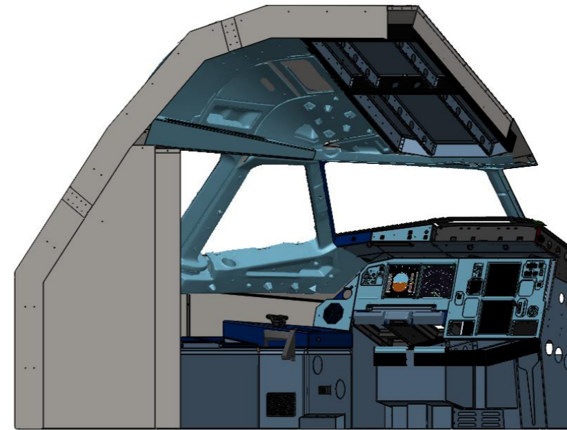
ISOMETRIC VIEW
