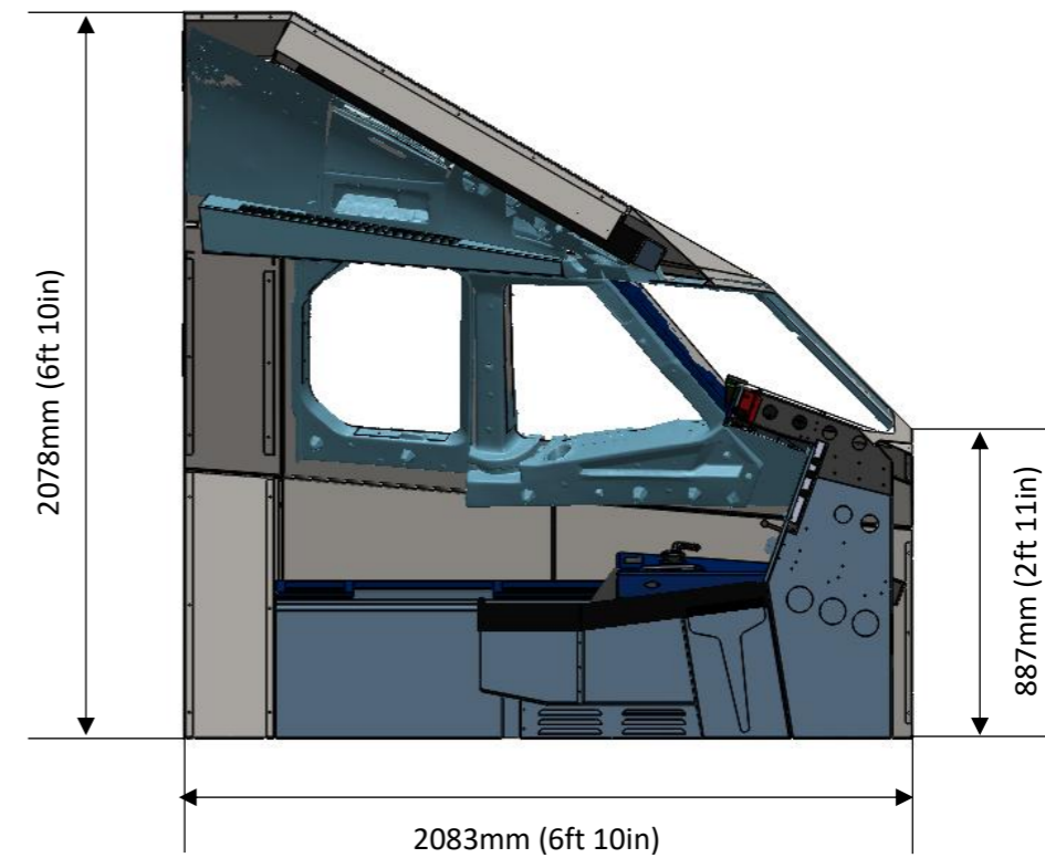
RIGHT VIEW
