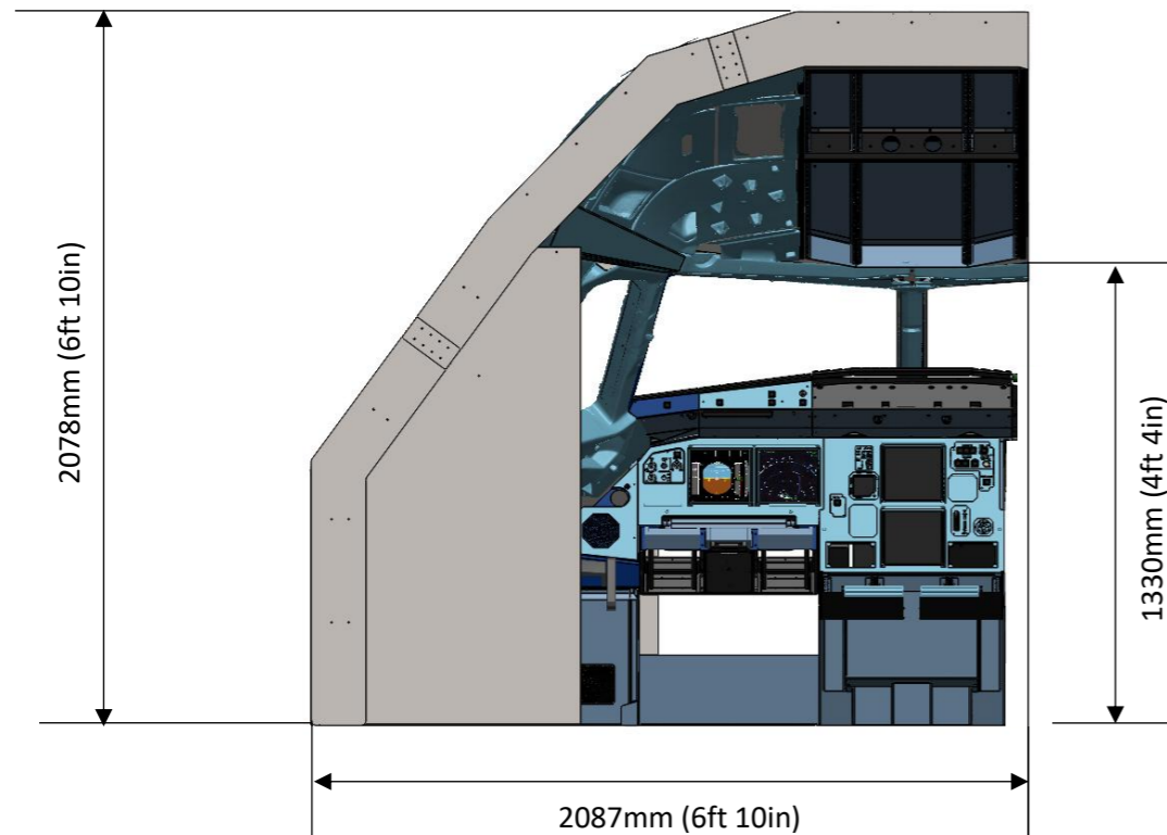
FRONT VIEW
